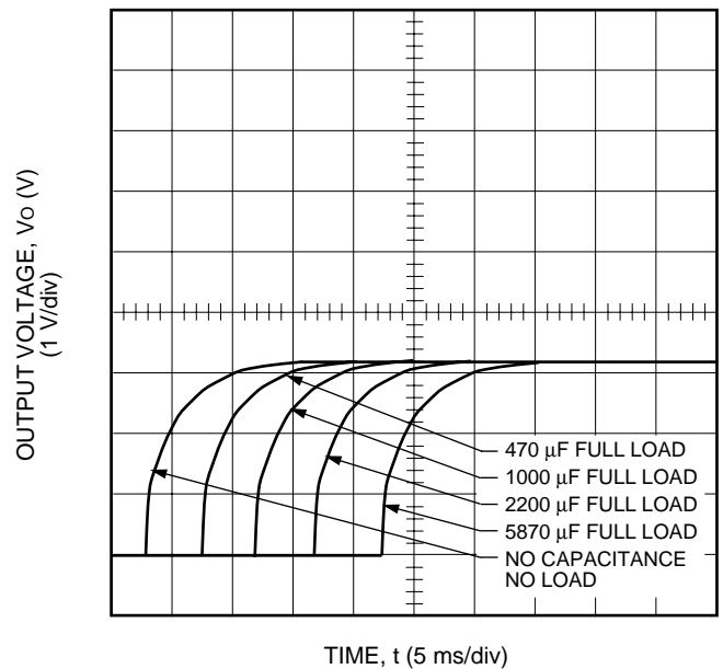
Note: Tested with a 10 \mu F aluminum and a 1.0 \mu F ceramic capacitor across the load. 8-2882 (F)
